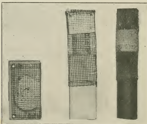
The Doolittle cage and two forms of the Miller cage.
