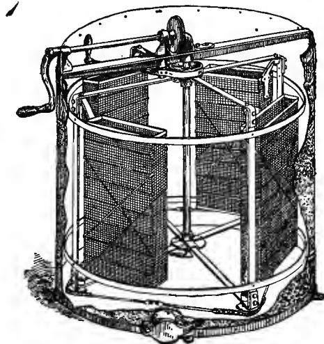
Fig. 21.—Extractor.
